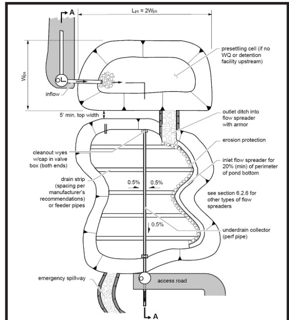
Figure 5-33: Plan View Schematic of Surface Sand Filter. Source: Washington.
