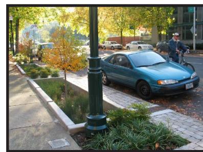
Figure 3-25 Bioretention planter boxes. Source Portland, OR BES.LID Center.
