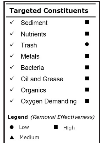
Figure 5-35: Green Roof Performance. Source – CASQA
