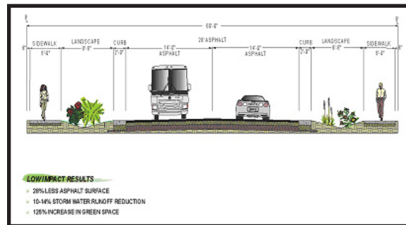
Figure 4-4 Suggested design standard for a rural 60’ wide road section. Source Logan, Utah.
