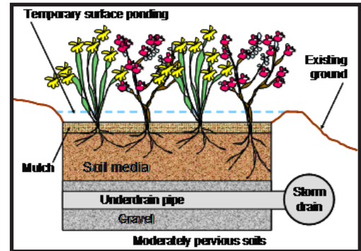
Figure 5-2 Typical cross section of a bioretention cell.
