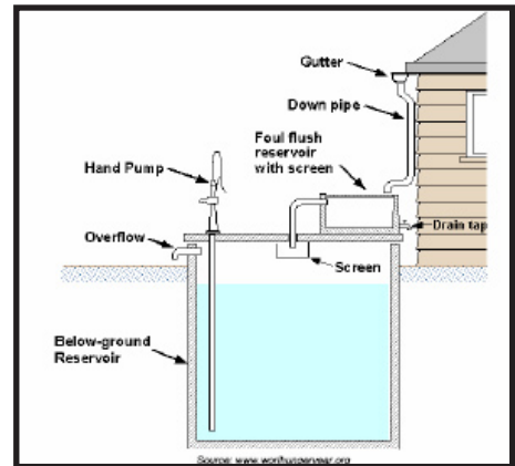
Figure 5-26: Underground Cistern
