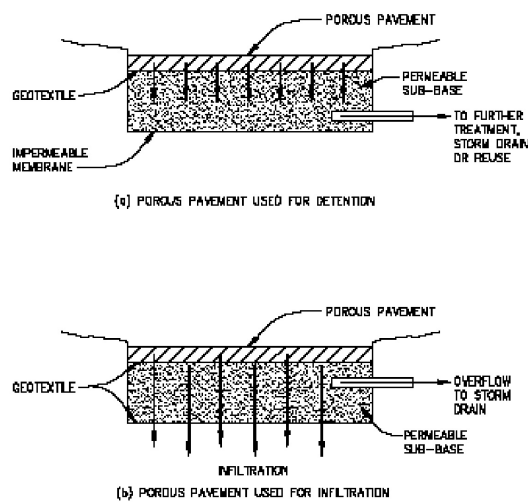
Figure 5-19 Cross-sections of typical permeable pavement installations. Source, City of Sacramento
