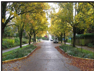
Figure 3-24 Street retrofit with bioretention cell on both sides of road. Source, Portland, OR BES.
