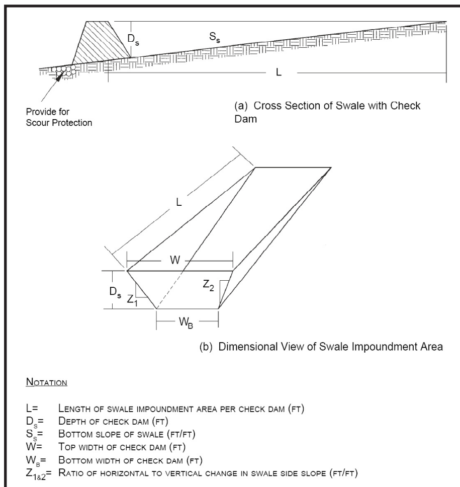
Figure 5-14 Cross section of swale with check dam (adapted from Maryland Department of Natural Resources, 1984).
