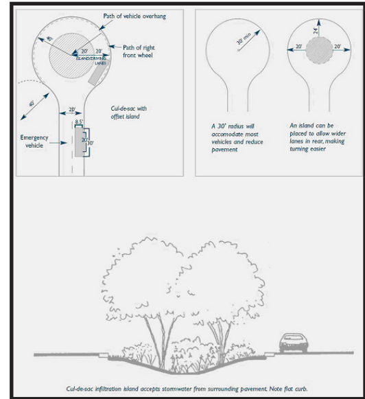
Figure 4-12 Example of Cul-de-sac design using bioretention. Source-Schuler 1995 and ASCE 1990. of-way. Source Portland, OR.
