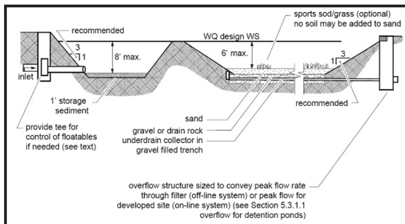
Figure 5-34: Section View Sand Filter Schematic. Source Washington
