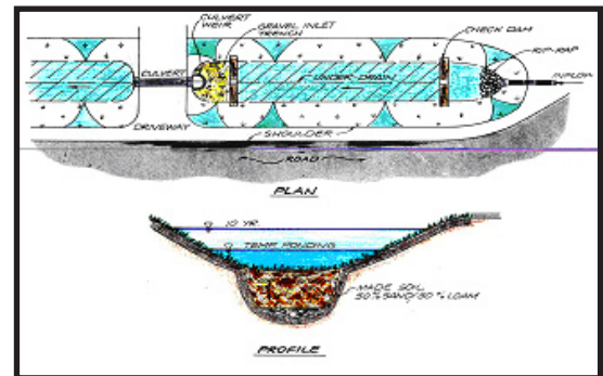
Figure 4-1 Example of a dry swale. Source Maryland Department of Environment.
