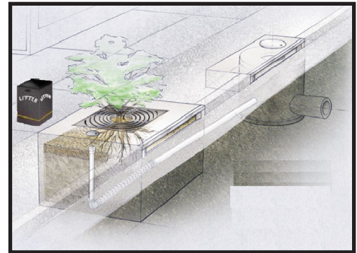
Figure 5-27 Tree Box Filter Upstream of Conventional Storm Drain. Source, Larry Coffman.
