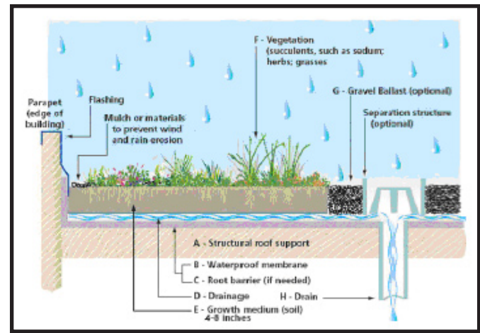
Figure 5-36 Typical green roof design cross-section. Source, LID Center.
