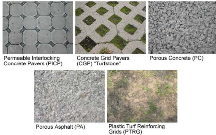
Figure 5-17: Various Permeable Pavement Systems. Source – NC State University.
