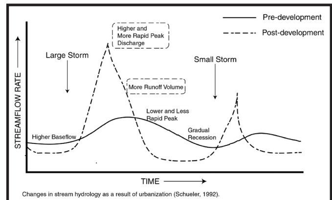
Figure 2-9 Comparison of pre- and post-development hydrographs. CWP 1992.
