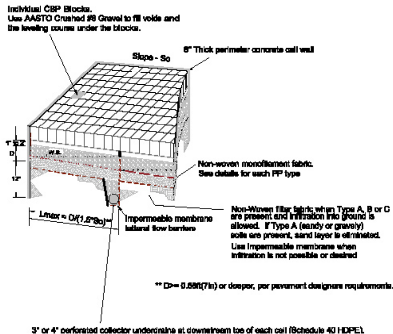
Figure 5-23 Porous Paver Block Design. Source Boulder Stormwater Management Plan
