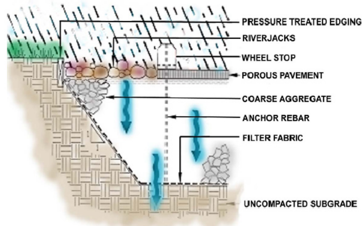
Figure 5-18 Cross section of Permeable pavement Parking Lot Design. Source Cahill and Associates.
