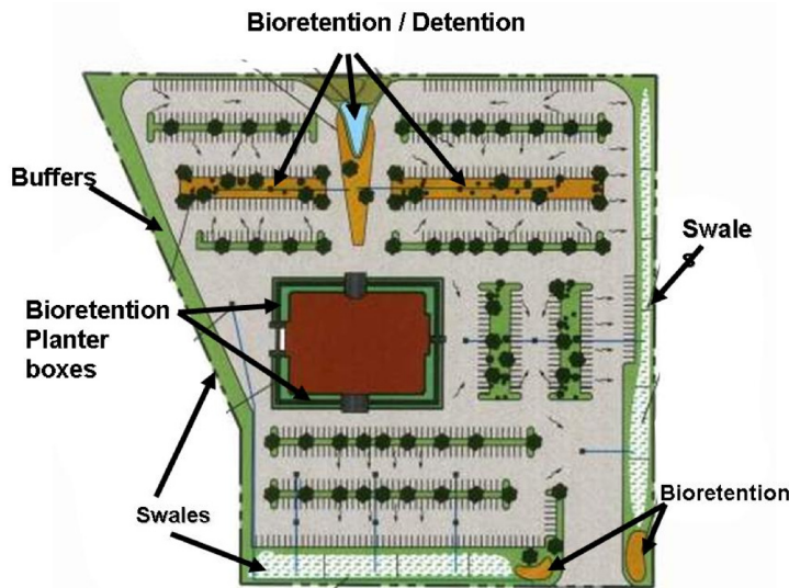
Figure 2-15 LID Design for a High Density Residential Site – This figure shows a residential high-rise development where LID techniques were applied throughout the parking area and perimeter landscape features.
