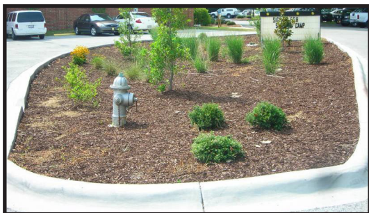
Figure 3-9 Completed porous parking and bioretention area at YMCA. Source NCSU.
