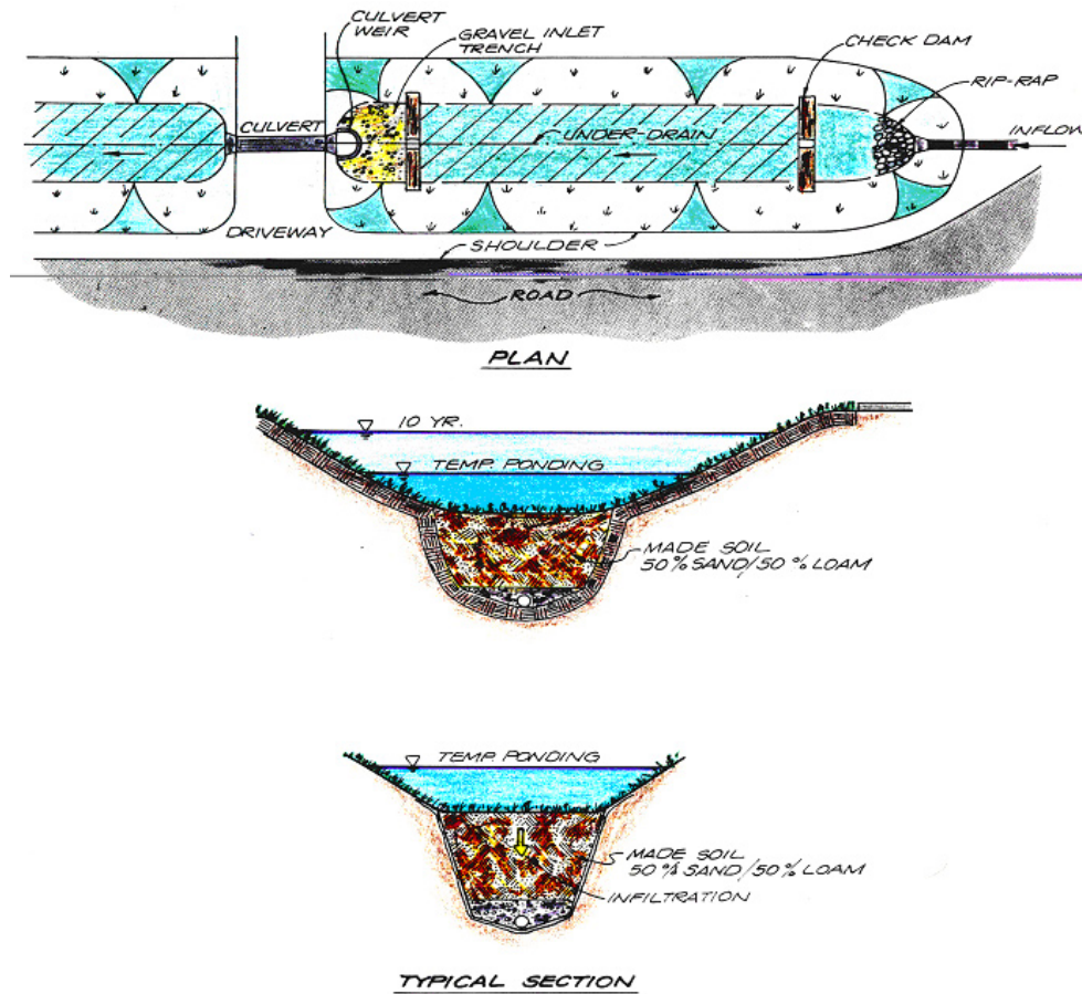
Figure 5-15 Infiltration Swale. Source, Maryland 2000 Design Manual.
