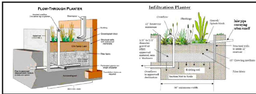
Figure 5-30: Stormwater Planters
