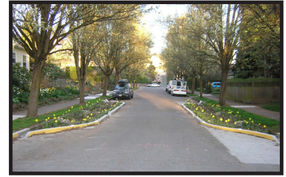
Figure 4-8 Bioretention cells used for both stormwater treatment and traffic calming. Source Portland.
