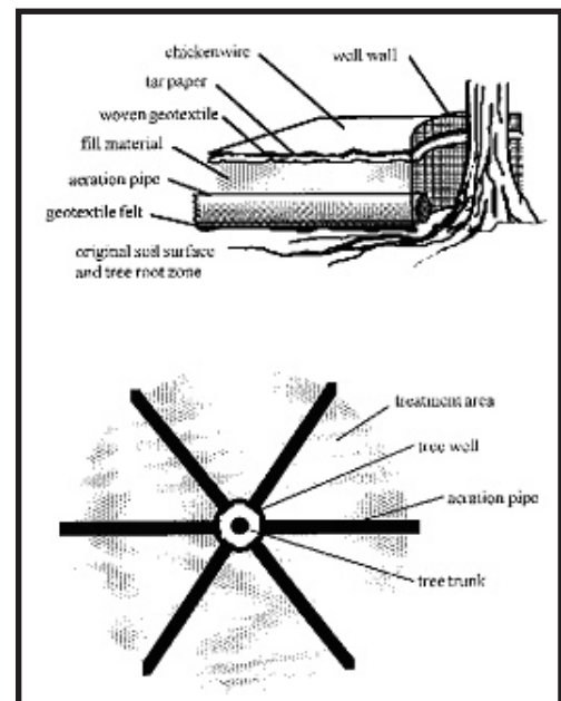
Figure 6-1: Radial Root Aeration System
