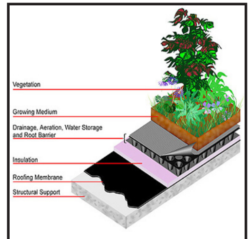
Figure 5-35 Typical green roof design elements. Source, LID Center.
