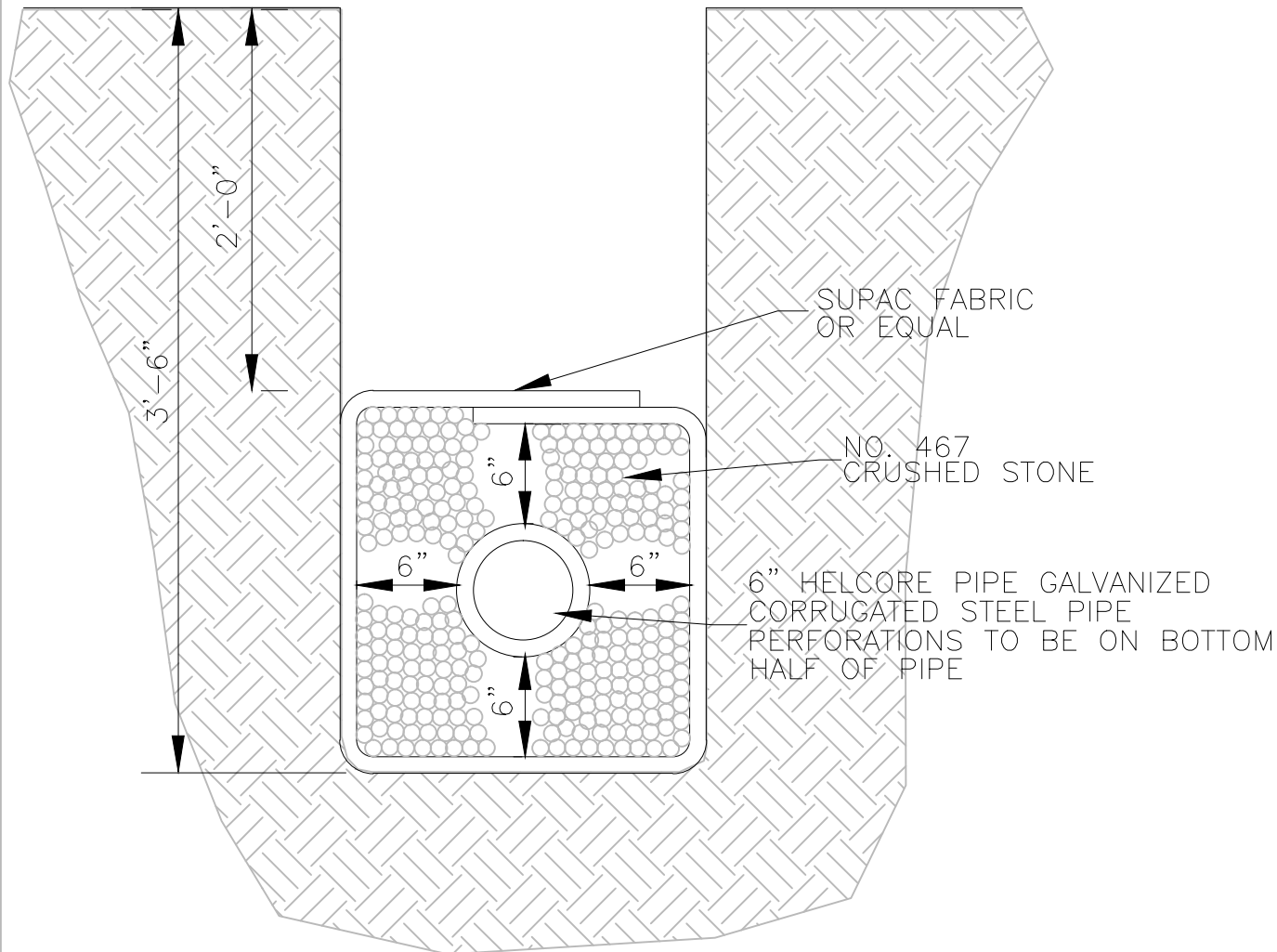
TYPICAL SECTION
